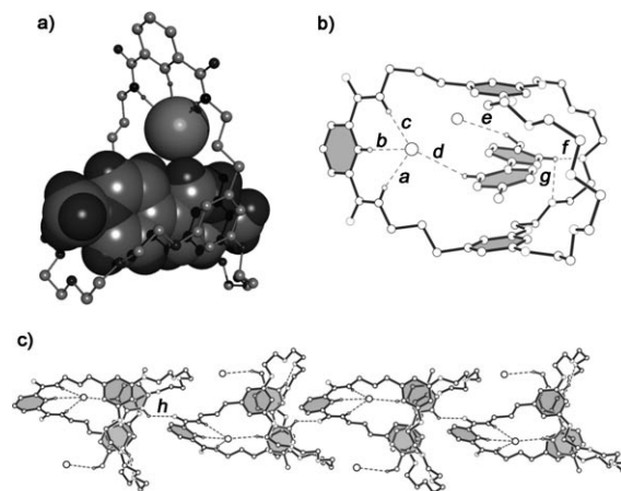
Figure 8. Views of the X-ray crystal structure of the 3g-2b complex. a) 3g is shown as a ball and stick model and chloride and bipyridinium dication are shown as space-filling models. b) Ball and stick representation of the 3g-2b complex. c) Ball and stick representation of the packing structure of the 3g-2b complex. Noninteracting hydrogen atoms have been omitted for clarity. Hydrogen bond parameters: \text{H}\cdots\text{O}(\text{F}, \text{Cl}) distance [ \text{\AA} ], \text{C}(\text{N})\cdots\text{O}(\text{Cl}) angle [ ^\circ ], \text{C}(\text{N})\cdots\text{O}(\text{Cl}) distance [ \text{\AA} ]. a ) 2.58, 166, 3.42, b ) 2.57, 169, 3.49, c ) 2.51, 161, 3.34, d ) 2.80, 141, 3.58, e ) 2.83, 160, 3.74, f ) 2.34, 156, 3.21, g ) 2.56, 103, 2.92, and h ) 2.40, 129, 3.07. Face-to-face \pi -stacking parameters: centroid-centroid distances [ \text{\AA} ]: 3.68, 4.80, 4.65, 3.84; ring plane/ring plane inclinations [ ^\circ ]: 7.7, 22.3, 9.07, 13.9.
