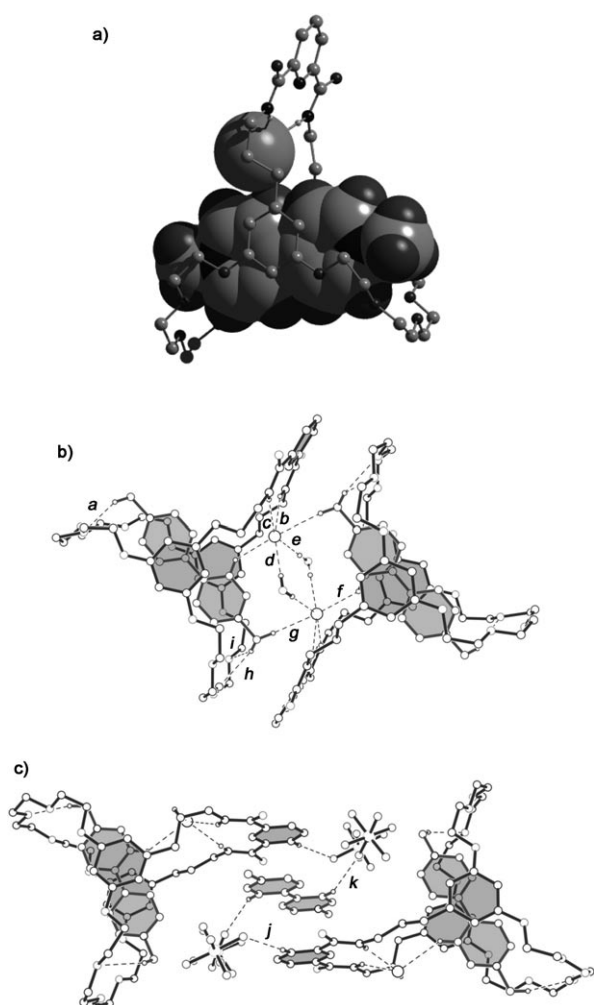
Figure 5. Views of the X-ray crystal structure of the 3c · 2a · 2b complex. a) 3c is shown as a ball and stick model and chloride and bipyridinium dication are shown as space-filling models. b) and c) Ball and stick representation of the packing of two adjacent cryptand/paraquat complexes in the unit cell in different directions. Noninteracting hydrogen atoms have been omitted for clarity. Hydrogen bond parameters: \text{H}\cdots\text{O}(\text{F}, \text{Cl}) distance [Å], \text{C}(\text{N})\text{-H}\cdots\text{O}(\text{F}, \text{Cl}) angle [°], \text{C}(\text{N})\cdots\text{O}(\text{F}, \text{Cl}) distance [Å]. a) 2.75, 143, 3.57, b) 2.56, 154, 3.35, c) 2.50, 151, 3.27, d) 2.38, 178, 3.23, e) 2.33, 178, 3.18, f) 2.69, 142, 3.47, g) 2.91, 132, 3.63, h) 2.54, 129, 3.23, i) 2.49, 136, 3.35, j) 2.70, 151, 3.91, and k) 2.49, 149, 3.91. Face-to-face \pi -stacking parameters: centroid-centroid distances [Å]: 4.60, 3.8, 4.49, 3.69; ring plane/ring plane inclinations [°]: 5.0, 6.0, 1.82, 1.19.
