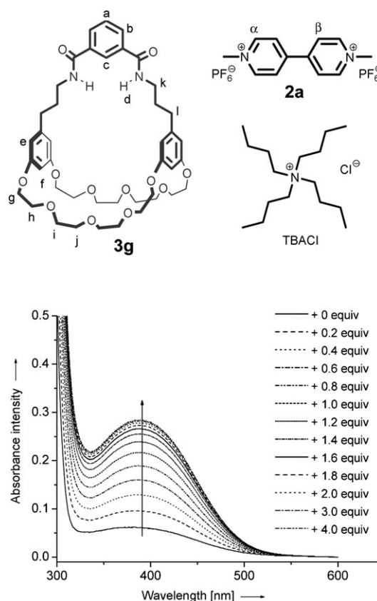
Figure 6. Absorbance spectral changes of an equimolar solution (2.00 mL) of 3g (0.500 mM) and 2a (0.500 mM) upon addition of TBACl (from 0 to 2.00 mM).
