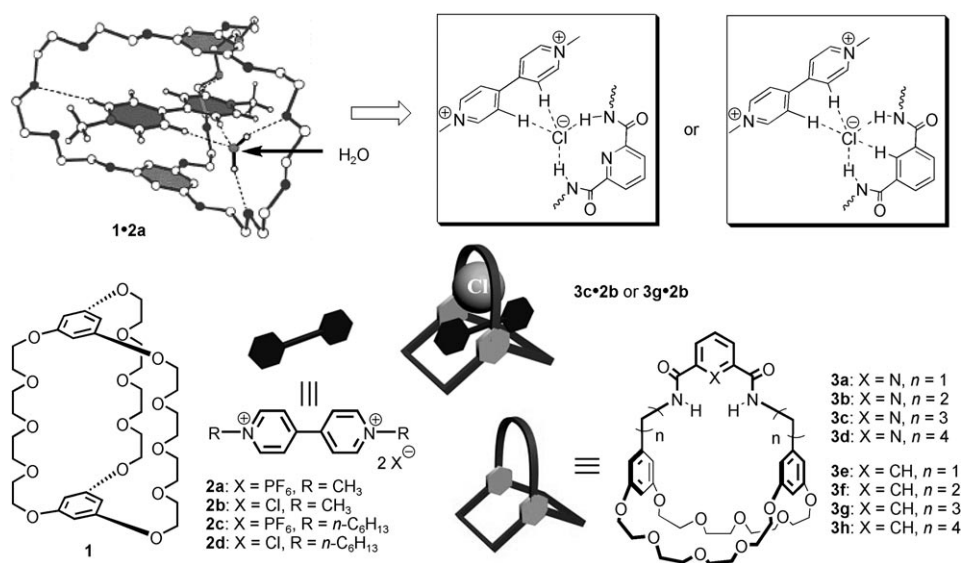
Figure 1. Compounds used in this study, together with the X-ray crystal structure of the 1·2a·H 2 O complex.
