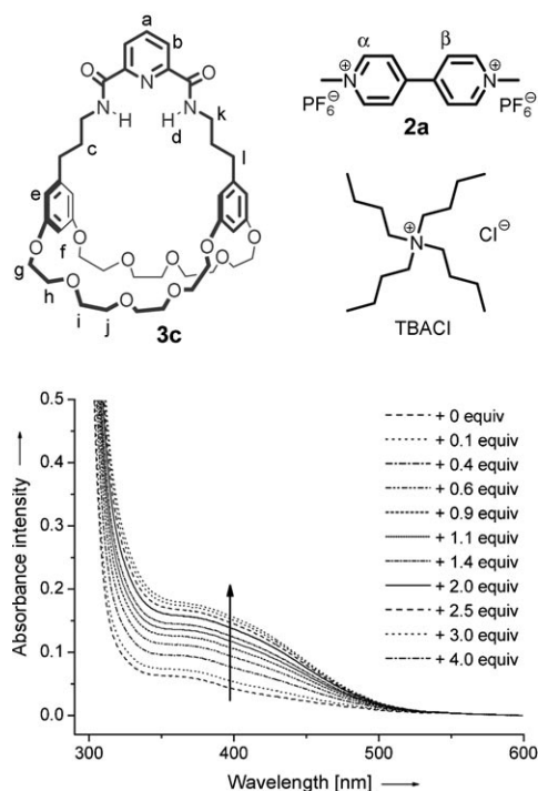
Figure 3. Absorbance spectral changes of an equimolar solution (2.00 mL) of 3c (0.500 mM) and 2a (0.500 mM) upon addition of TBACl (from 0 to 2.00 mM).
