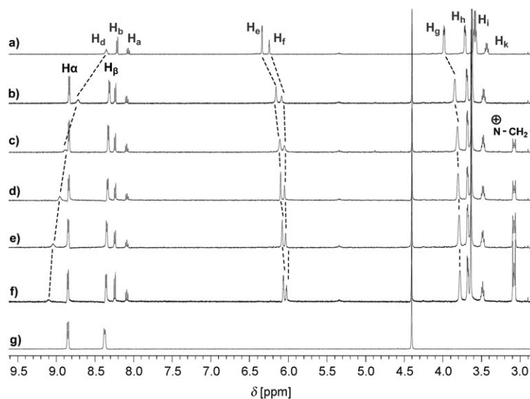
Figure 4. Partial ^1H NMR spectra (500 MHz, CD_3CN , 20 °C) of: a) 3c (0.500 mM), b) an equimolar mixture of 3c (0.500 mM) and 2a (0.500 mM), c) (b)+TBACl (0.180 mM), d) (b)+TBACl (0.220 mM), e) (b)+TBACl (0.500 mM), f) (b)+TBACl (1.00 mM), and g) 2a (1.00 mM).
