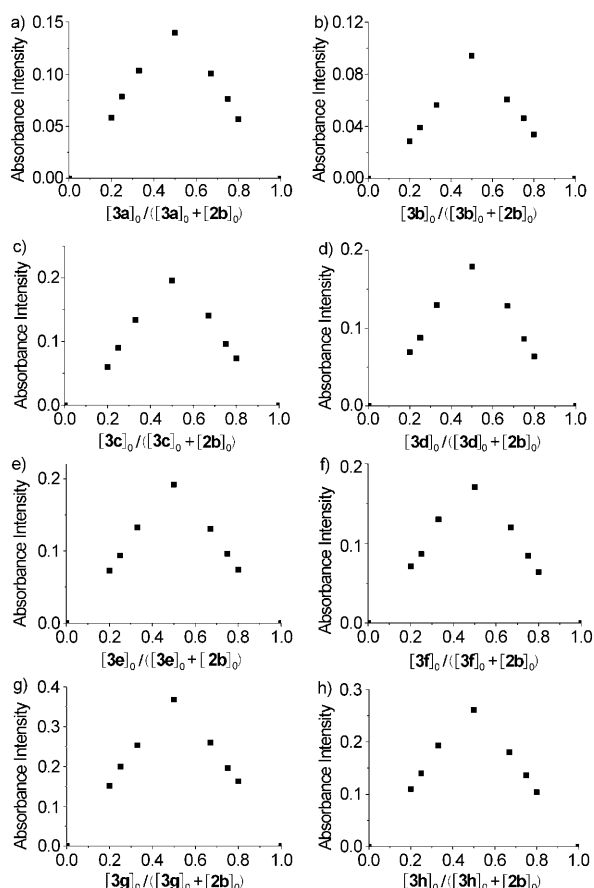
Figure 2. Job plots showing the 1:1 stoichiometries of the complexes formed between hosts 3 and 2b in \text{CHCl}_3/\text{CH}_3\text{OH} (1:1). The absorbance intensities at \lambda = 388 nm (the host–guest charge-transfer band) were plotted against the mole fractions of the hosts. [3]^0 and [2b]^0 are initial concentrations of 3 and 2b , respectively. a) [3a]^0 + [2b]^0 = 2.00 mM; b) [3b]^0 + [2b]^0 = 2.00 mM; c) [3c]^0 + [2b]^0 = 1.00 mM; d) [3d]^0 + [2b]^0 = 1.00 mM; e) [3e]^0 + [2b]^0 = 1.00 mM; f) [3f]^0 + [2b]^0 = 1.00 mM; g) [3g]^0 + [2b]^0 = 1.00 mM; h) [3h]^0 + [2b]^0 = 1.00 mM.
