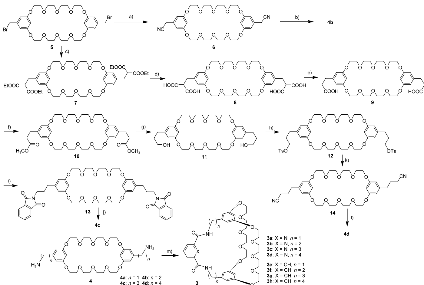
Scheme 1. Synthesis of cryptand hosts 3 , based on bis( m -phenylene)-[32]crown-10: a) NaCN, THF/H 2 O, reflux, 85%; b) borane methylsulfide, THF, reflux, 84%; c) CH 2 (COOEt) 2 , NaH, THF, 98%; d) i) NaOH (2 M), EtOH, reflux; ii) HCl, H 2 O, 99% (two steps); e) 140 °C, N 2 , 75%; f) H 2 SO 4 , CH 3 OH, 89%; g) LiAlH 4 , THF, 92%; h) TsCl, Et 3 N, CH 2 Cl 2 , 73%; i) potassium phthalimide, DMF, 90 °C, 93%; j) i) hydrazine monohydrate, CH 3 OH, reflux; ii) HCl, H 2 O, iii) NaOH, H 2 O, 90% (three steps); k) NaCN, DMF, 80 °C, 92%; l) borane methylsulfide, THF, reflux, 88%; m) isophthaloyl dichloride or 2,6-dipyridinecarbonyl dichloride, Et 3 N, CH 2 Cl 2 , 6–54%.
