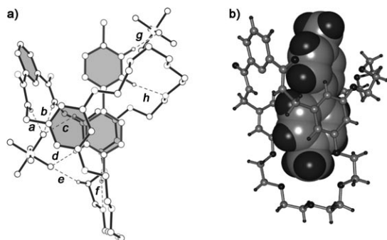
Figure 9. Views of the X-ray crystal structure of the 3a-2a complex. a) Ball and stick representation of the 3a-2a complex. b) 3a is shown as a ball and stick model, and the bipyridinium cation is shown as a space-filling model. Noninteracting hydrogen atoms have been omitted for clarity. Hydrogen bond parameters: H...O(F, Cl) distance [Å], C(N)–H...O(Cl) angle [°], C(N)–H...O(Cl) distance [Å]. a ) 2.30, 156, 3.11, b ) 2.29, 146, 3.05, c ) 2.57, 123, 3.18, d ) 2.39, 163, 3.30, e ) 2.43, 159, 3.35, f ) 2.48, 141, 3.28, g ) 2.31, 162, 3.21, and h ) 2.34, 166, 3.25. Face-to-face \pi -stacking parameters: centroid–centroid distances [Å] 3.60, 5.25, 3.65, 5.57; ring-plane/ring-plane inclinations [°]: 4.5, 29.5, 0.64, 27.4.
