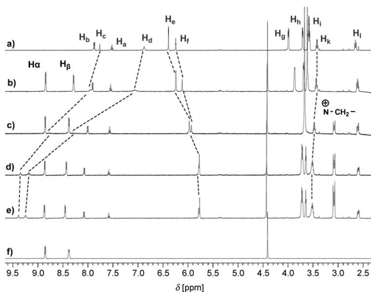
Figure 7. Partial ^1\text{H} NMR spectra (500 MHz, \text{CD}_3\text{CN} , 20^\circ\text{C} ) of: a) 3g (0.500 mM), b) an equimolar mixture of 3g (0.500 mM) and 2a (0.500 mM), c) (b)+TBACl (0.200 mM), d) (b)+TBACl (0.500 mM), e) (b)+TBACl (1.00 mM), and f) 2a (0.500 mM).
